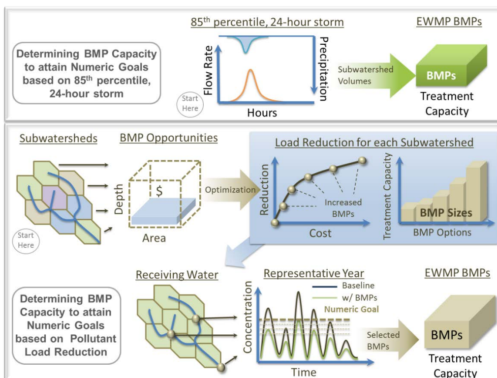
Figure A-15 Illustration of Screening Process to Compare the Load- and Volume-based Compliance Pathways
