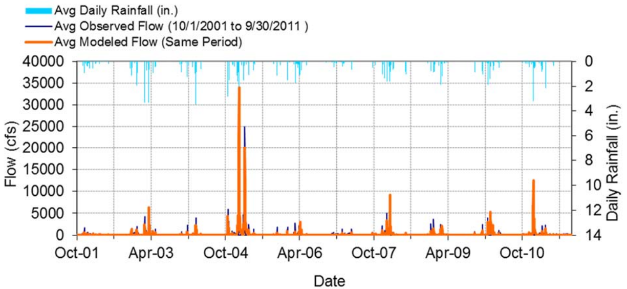
Figure 5-8 Mean daily flow for USGS 11087020 SAN GABRIEL R AB WHITTIER NARROWS DAM CA (10/1/2002 – 9/30/2011)
